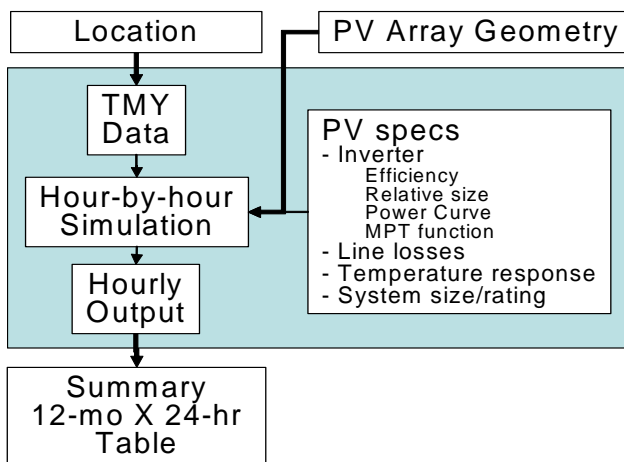
Fig.1: Input-output flowchart for time-series based PV simulations
